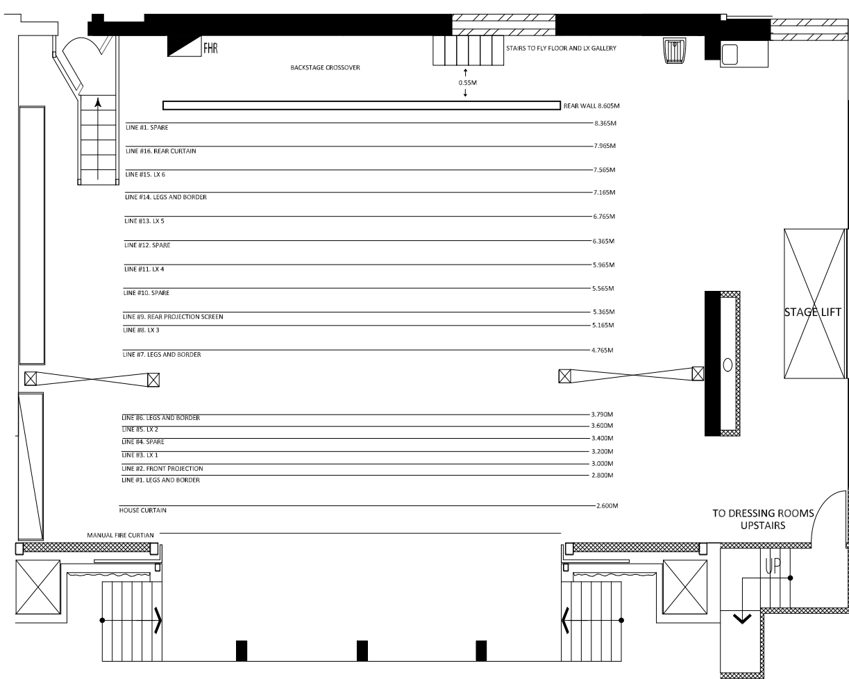
FLY TOWER SUPER STRUCTURE
